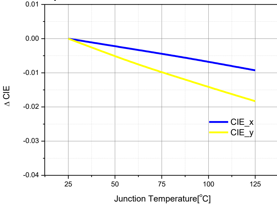
Junction Temperature vs. White ΔCIE at IF=1400mA
