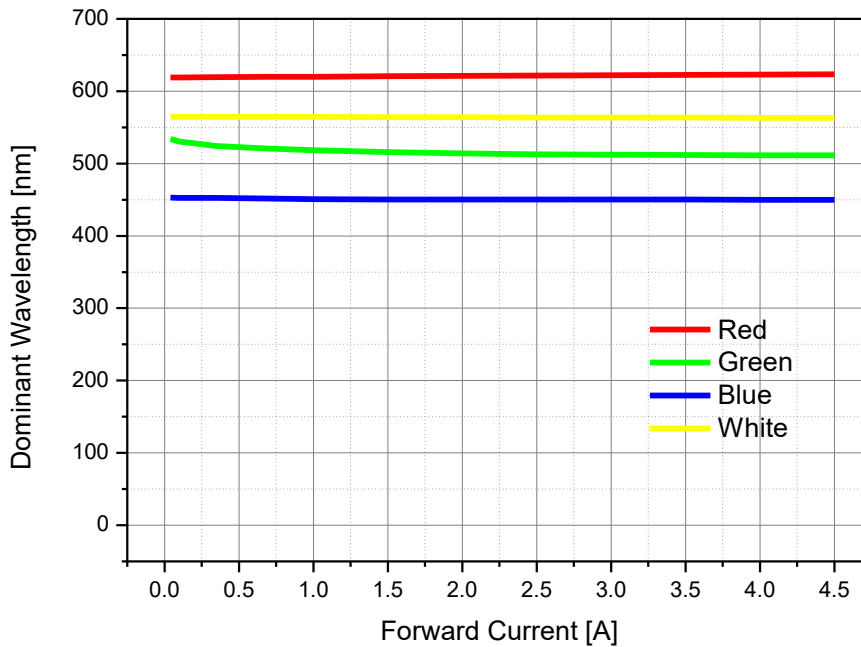
Forward Current vs Dominant Wavelength, T_j=25^\circ\text{C}
